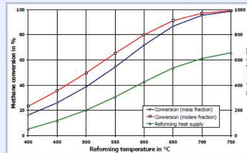
Methane conversion and heat demand of the reforming reaction (S/C=2.5, 2 kW LHV natural gas)
